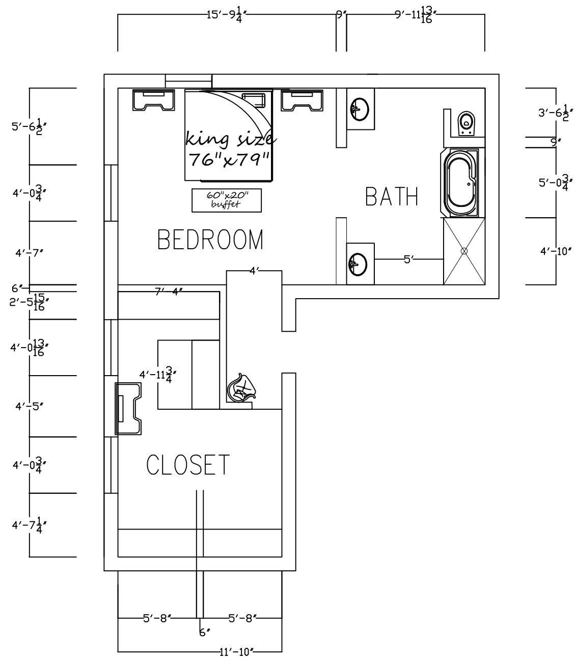
SANDI LITZINGER BEDROOM BATH FLOOR PLAN
